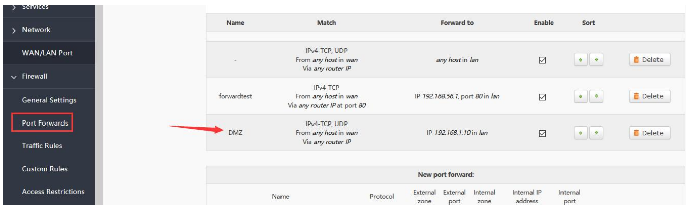
Figure48 DMZ setting2
