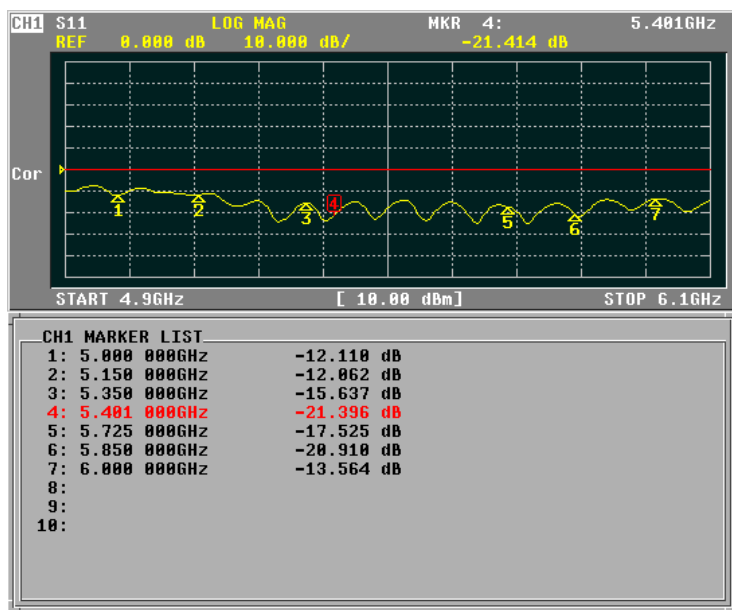
Return loss
