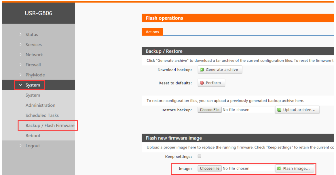
Figure 1 Webpage upgrading interface
